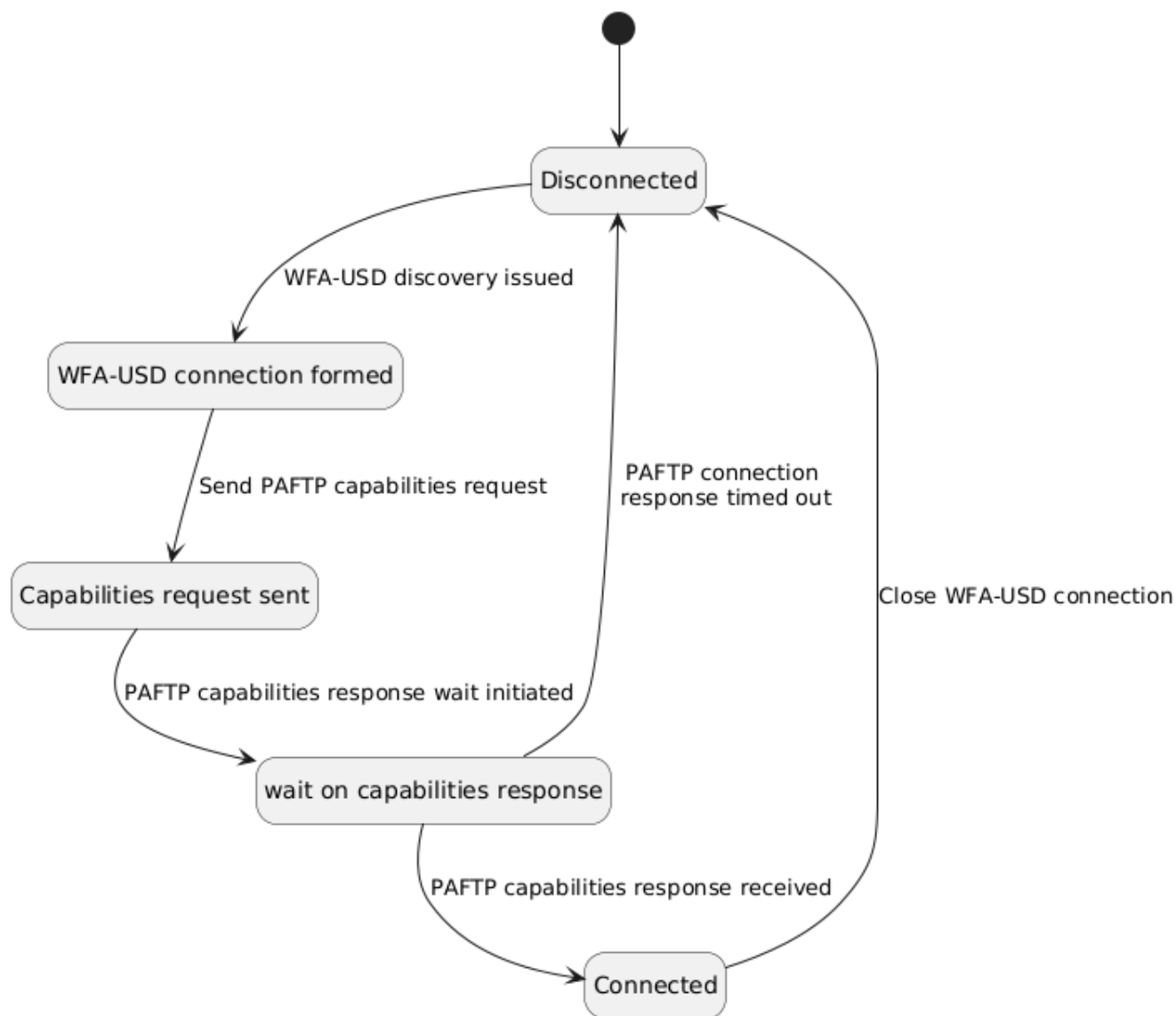
Figure 34. PAFTP session lifecycle for Commissioner
