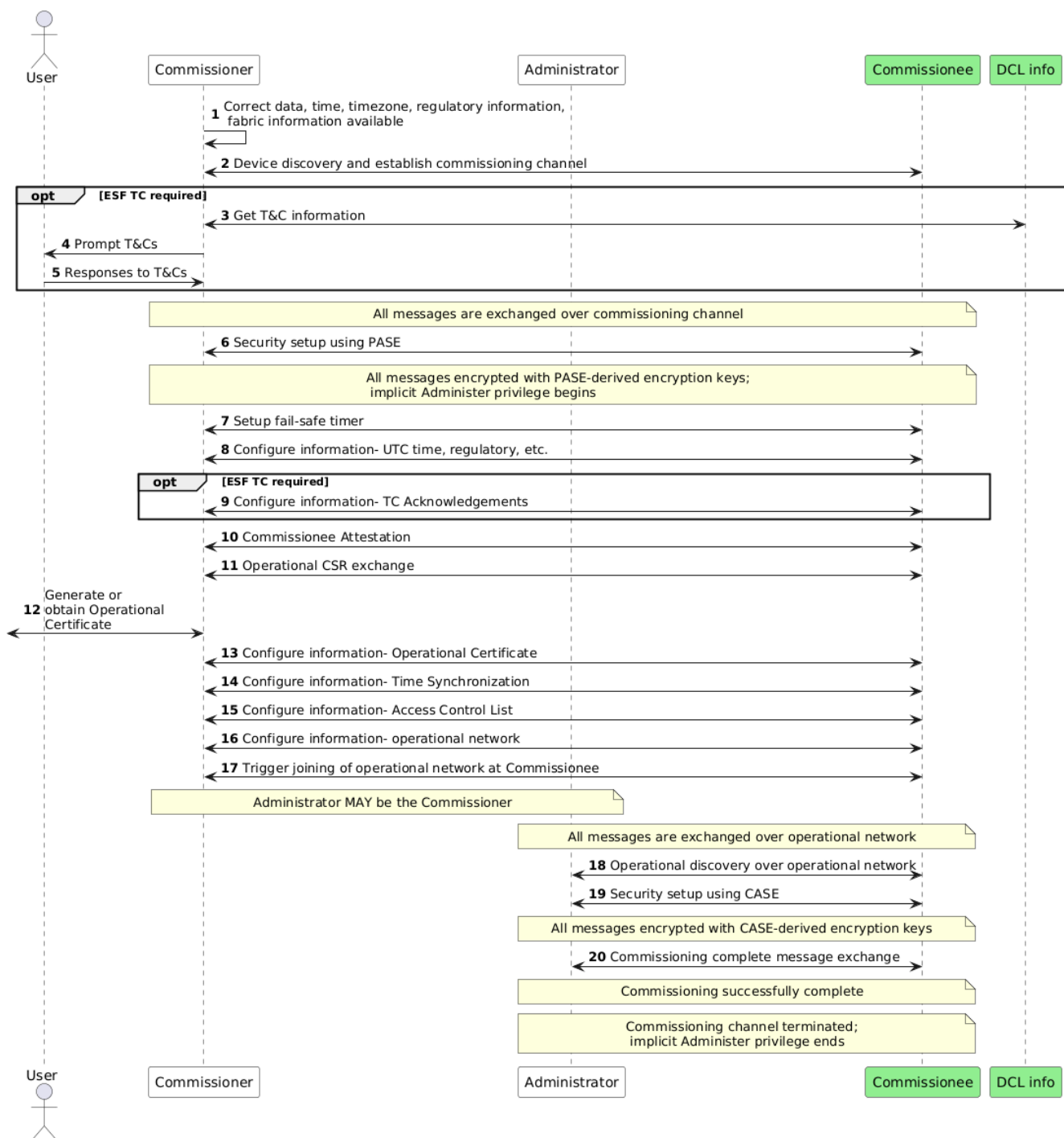
Figure 39. Concurrent connection commissioning flow
