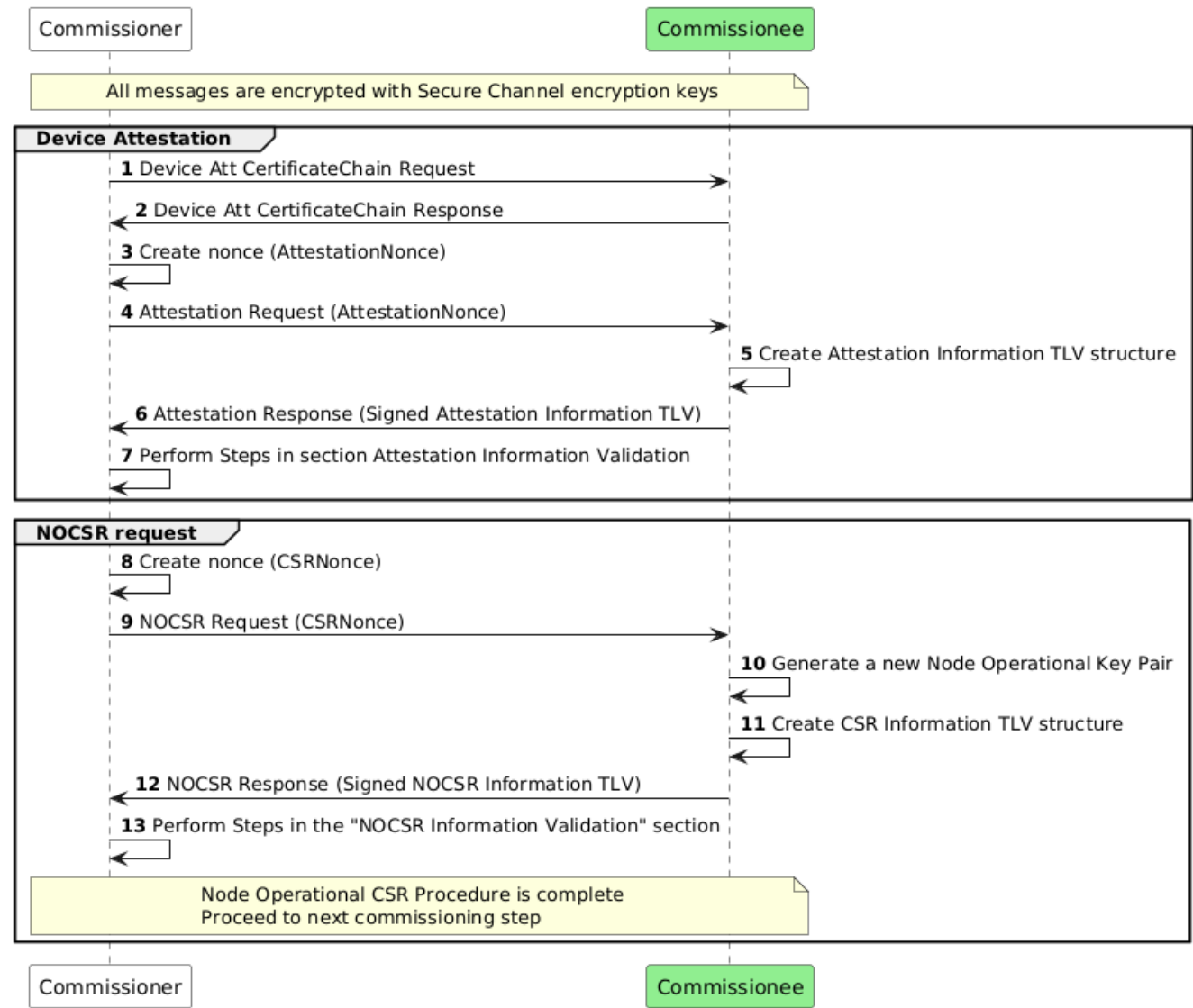
Figure 50. Node Operational Credentials flow
