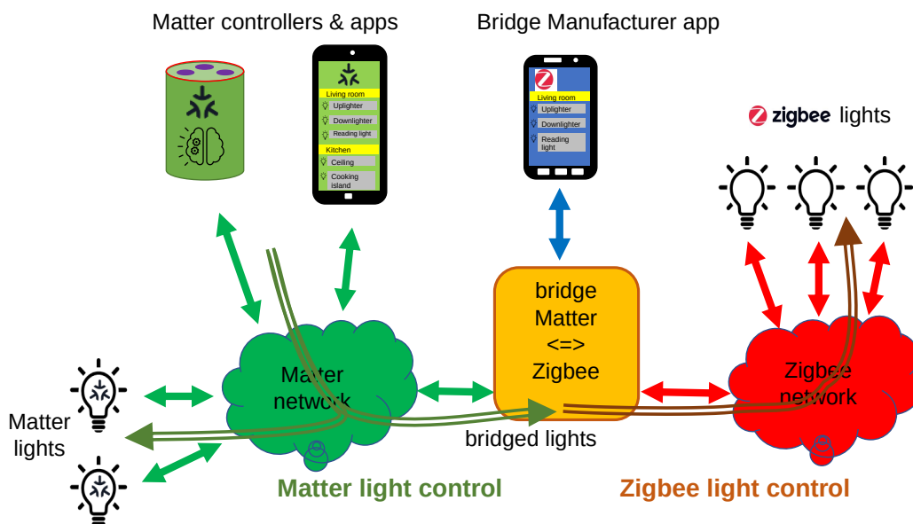
Figure 63. example of bridging lights
