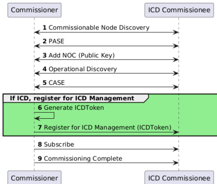
Figure 74. Commissioner Self-Registration to ICD
