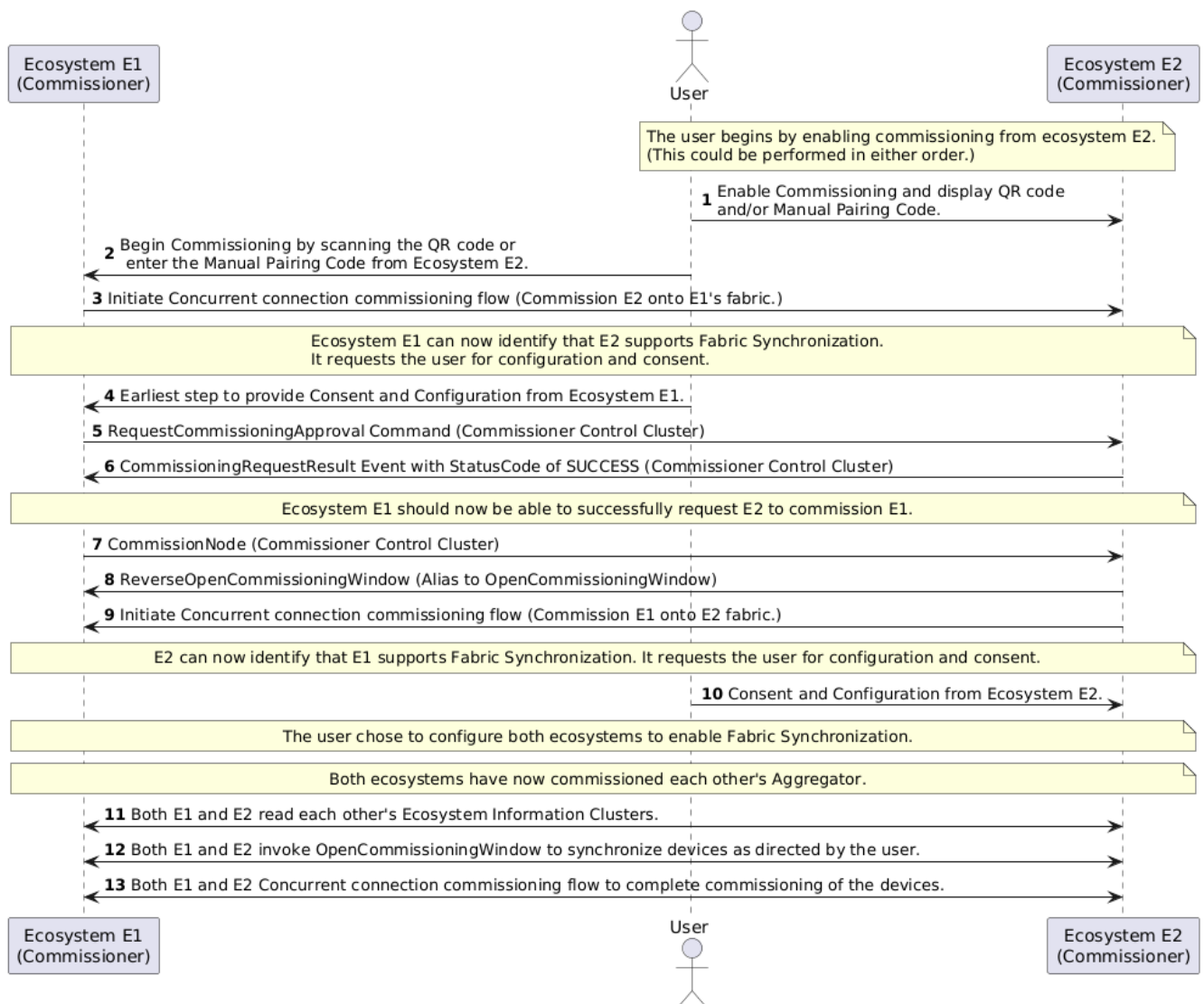
Figure 110. Fabric Synchronization Setup - Example Complete Flow.
