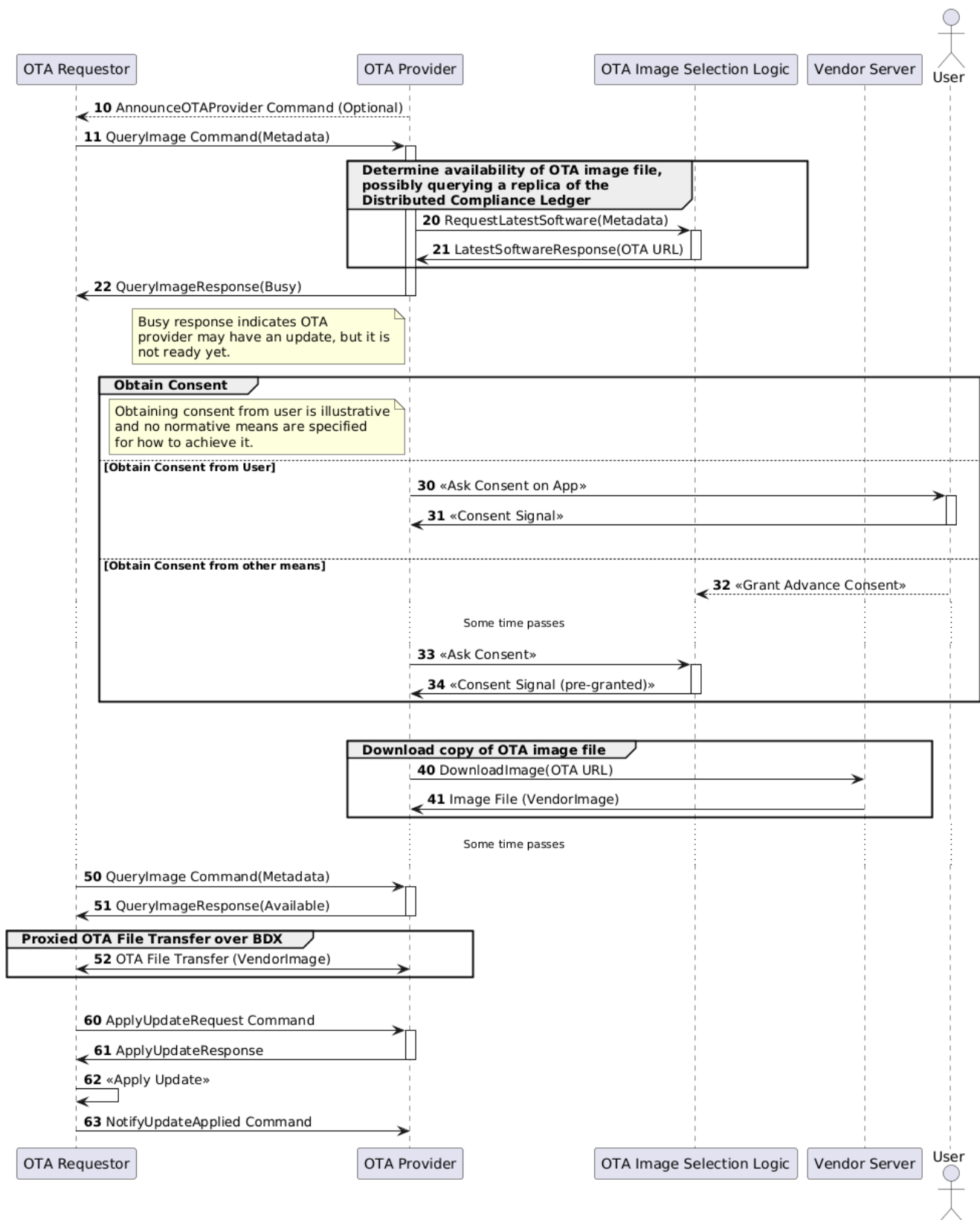
Figure 89. Detailed OTA Software Update Workflow
