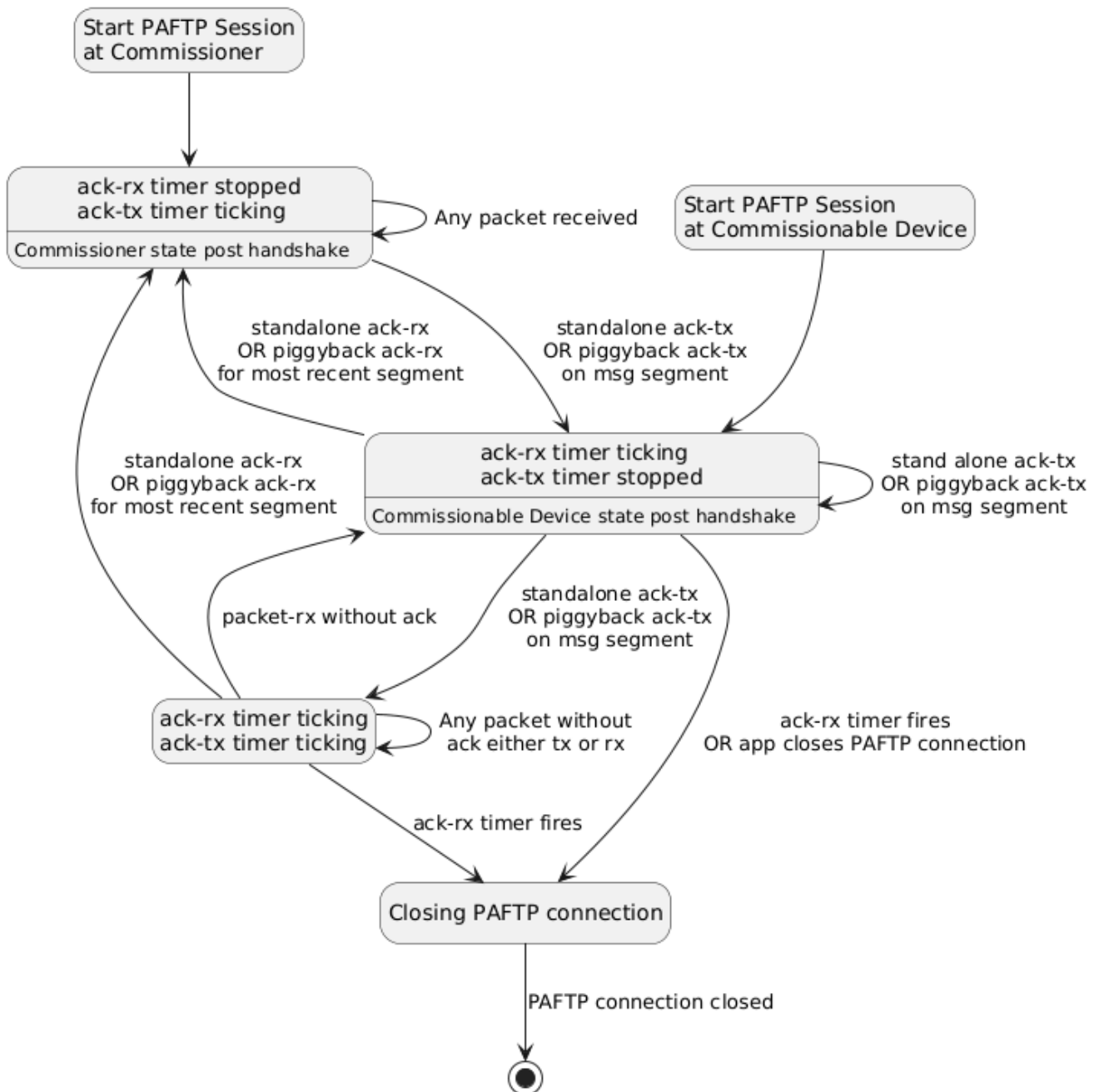
Figure 36. State diagram for PAFTP session post-establishment
