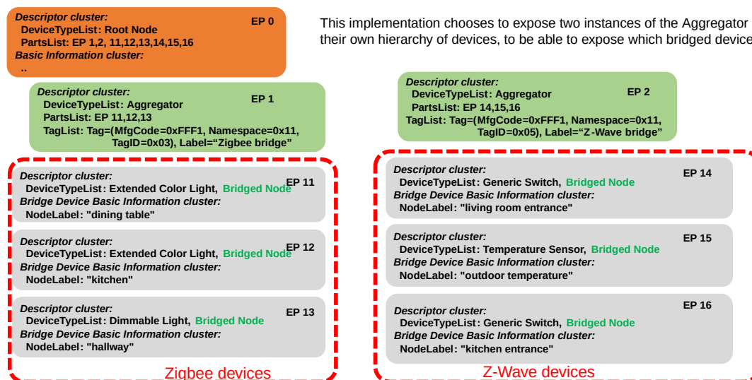
Figure 59. example of endpoints representing Bridged Devices from two technologies
