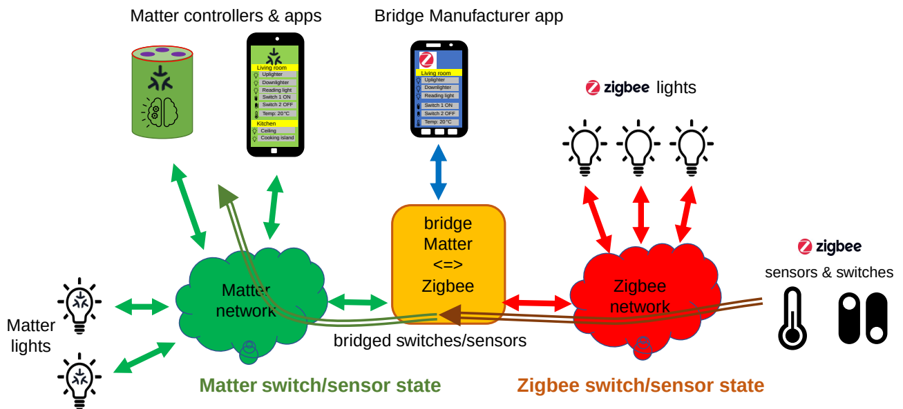
Figure 64. example of bridging switches and sensors
