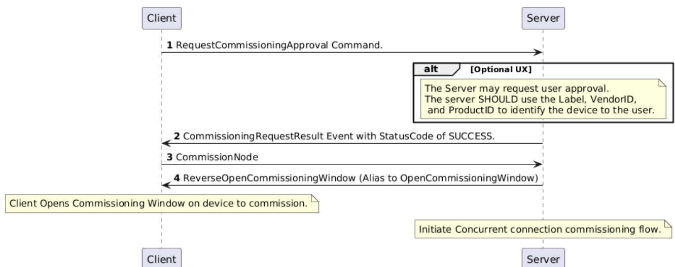
Figure 101. Commissioner Control Cluster - General Flow
