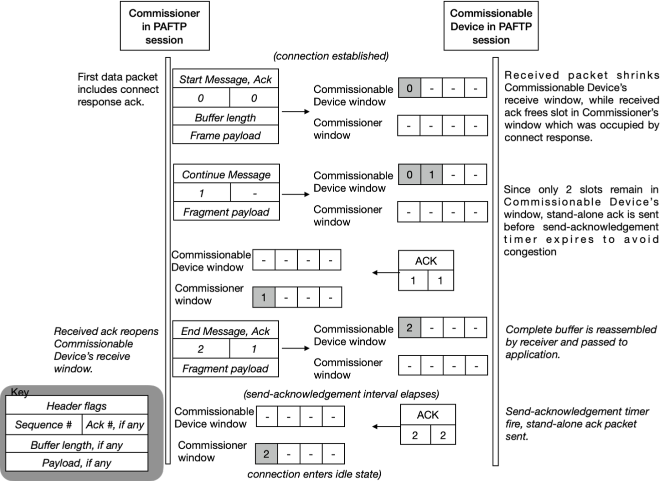
Figure 32. Example receive window scenario
