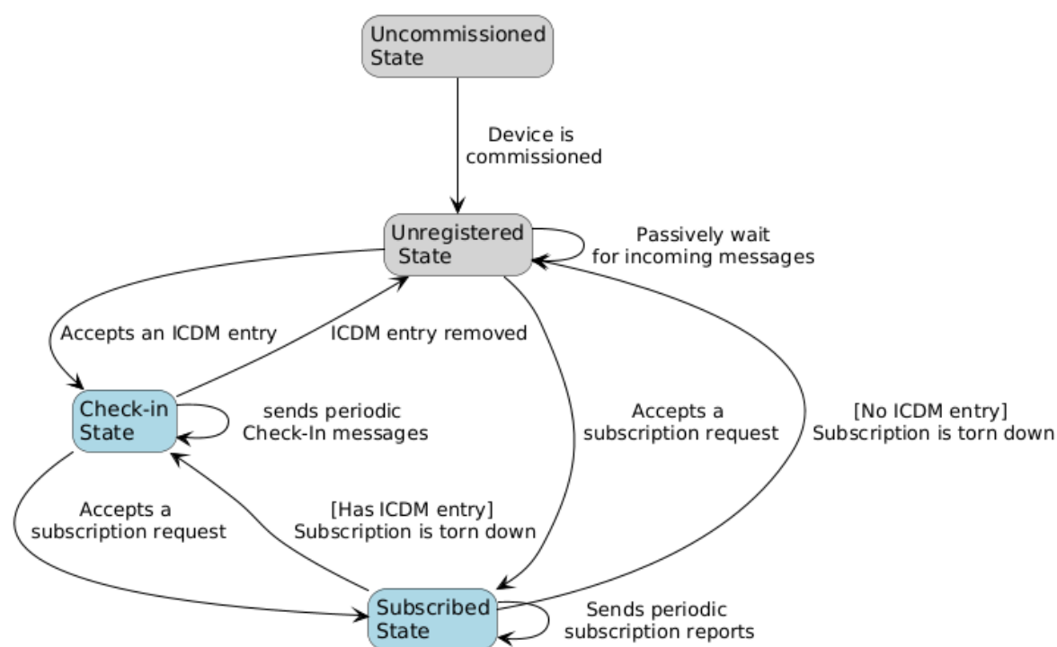
Figure 71. ICD State Machine
