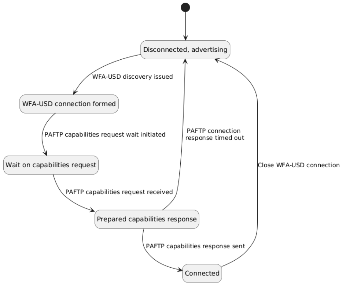
Figure 35. PAFTP session lifecycle for Commissionable Device
