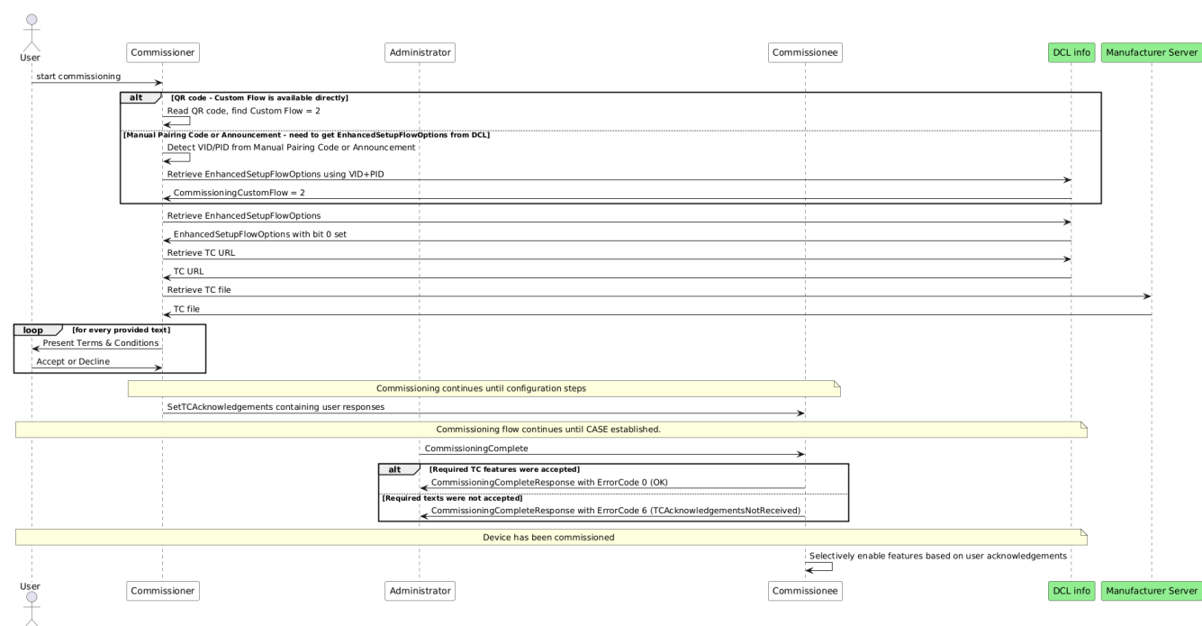
Figure 43. Enhanced Setup Flow TC commissioning sequence diagram
