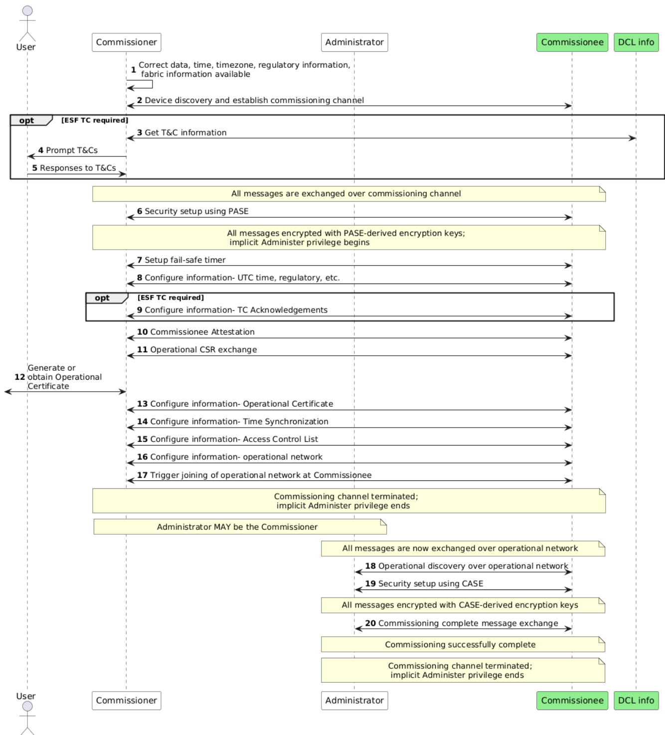
Figure 40. Non-concurrent connection commissioning flow
