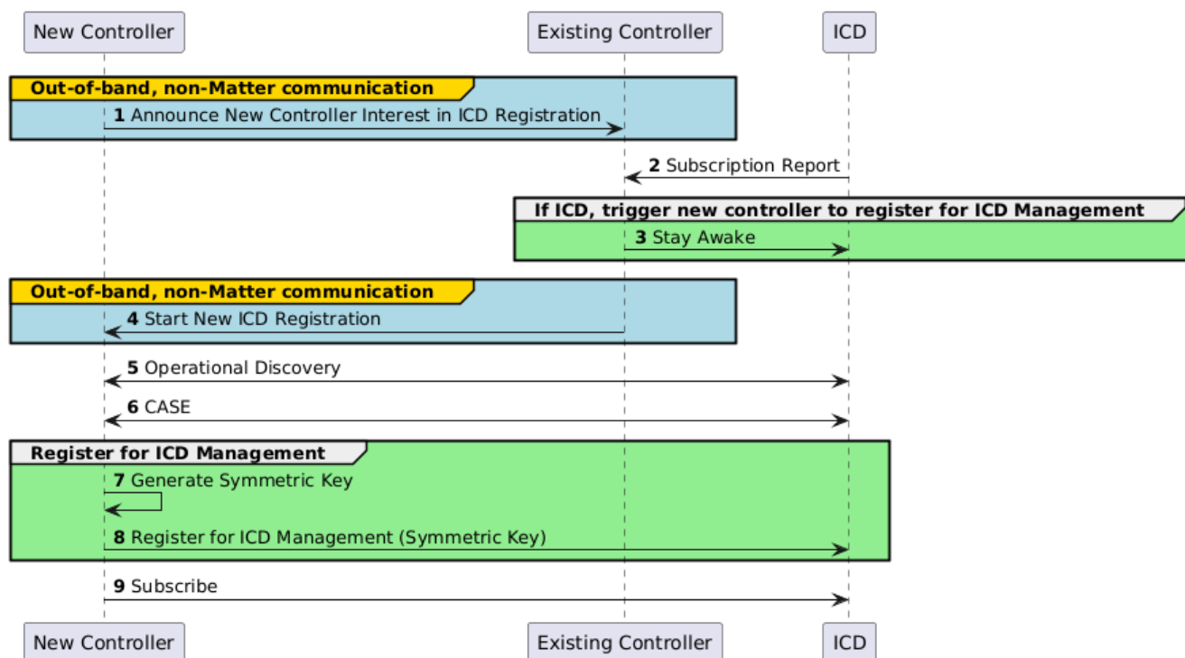
Figure 77. Infrastructure Assisted On-Demand Registration
