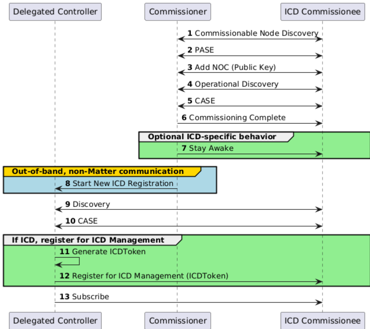
Figure 76. Delegated Controller Registration
