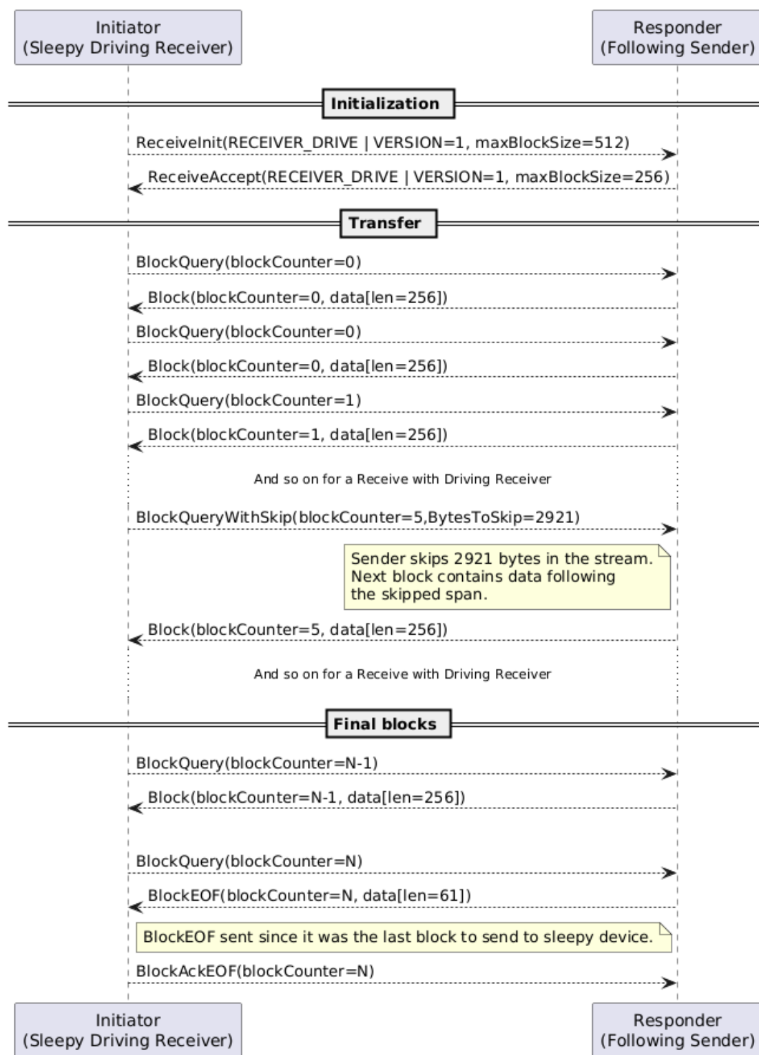
Figure 95. Synchronous file receiving by device acting as driving Receiver, including BlockQueryWithSkip
