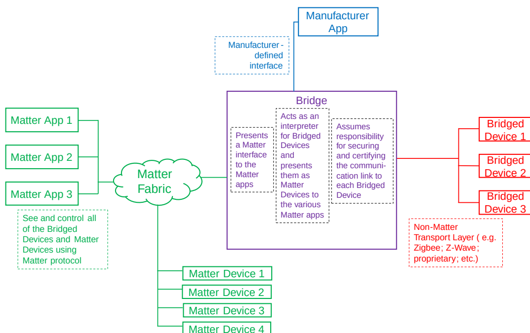
Figure 57. principle of bridging
