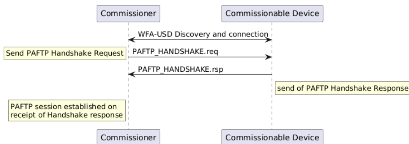
Figure 31. PAFTP session handshake
