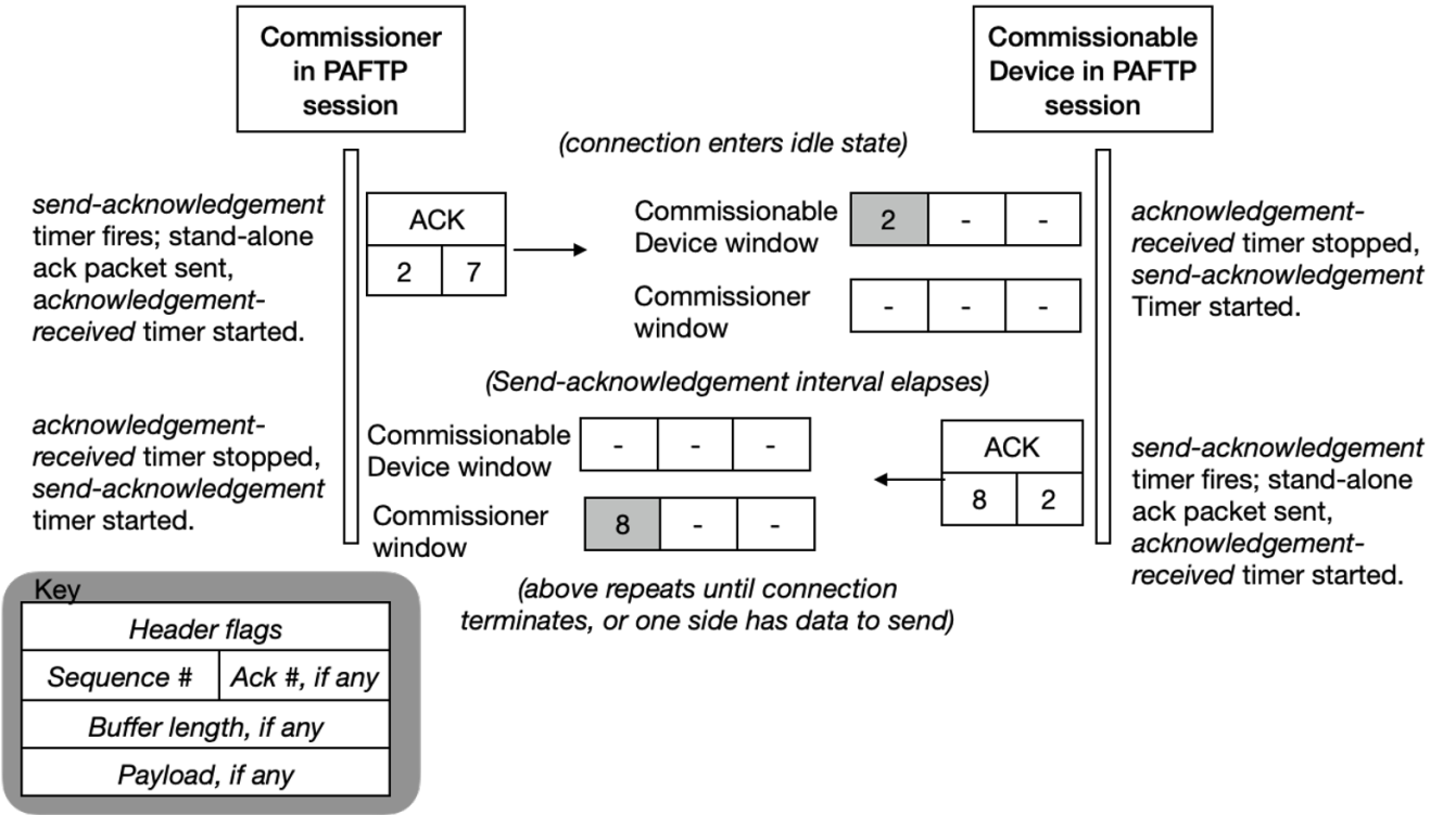
Figure 33. Idle connection scenario
