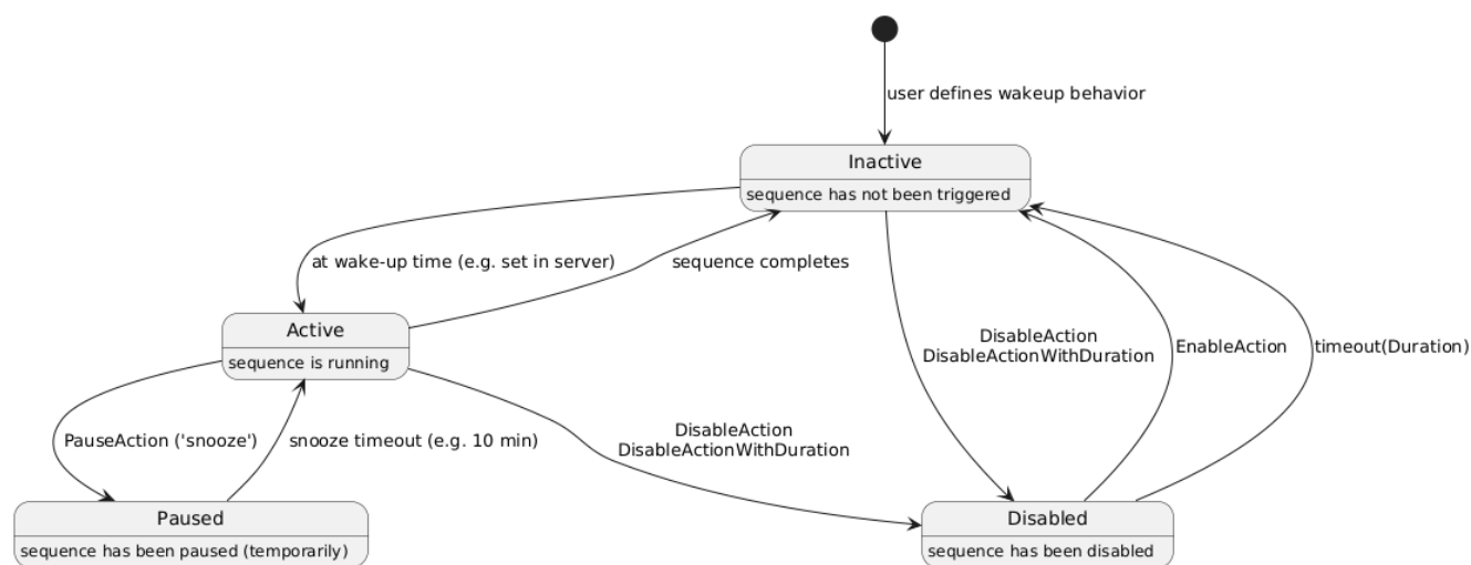
Figure 68. State diagram for example 'wake-up experience'
