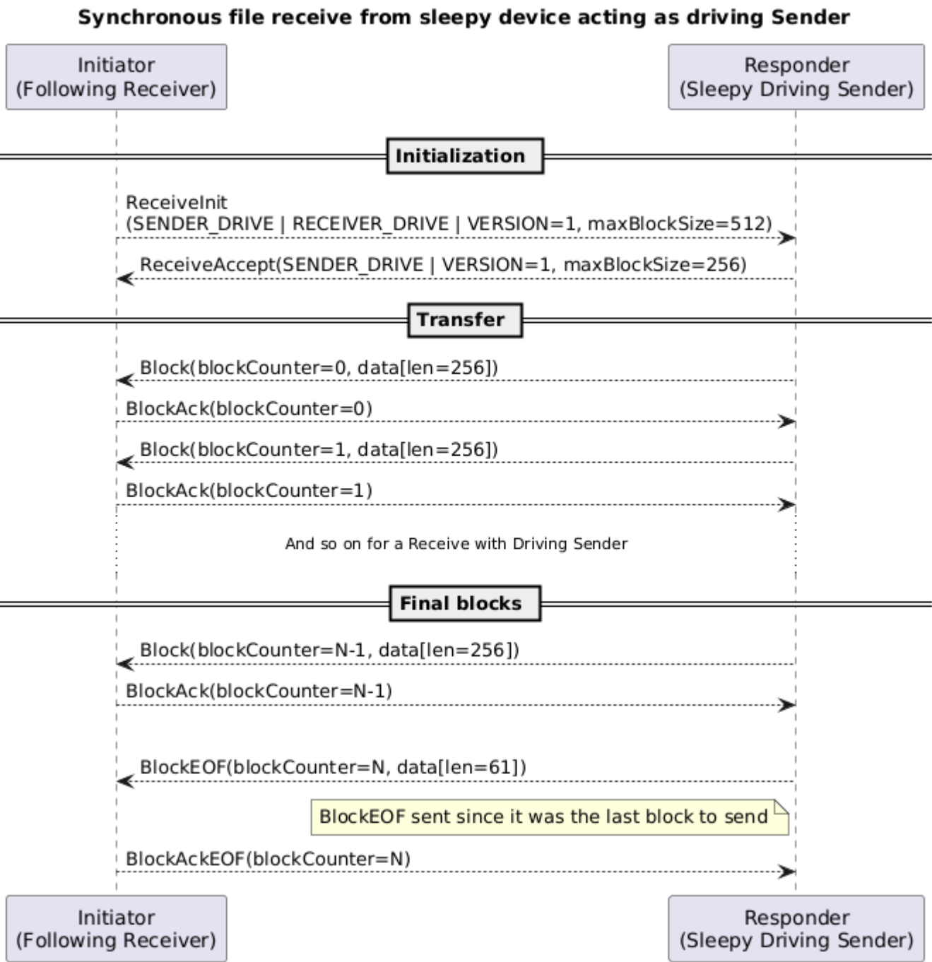
Figure 96. Synchronous file receive from sleepy device acting as driving Sender
