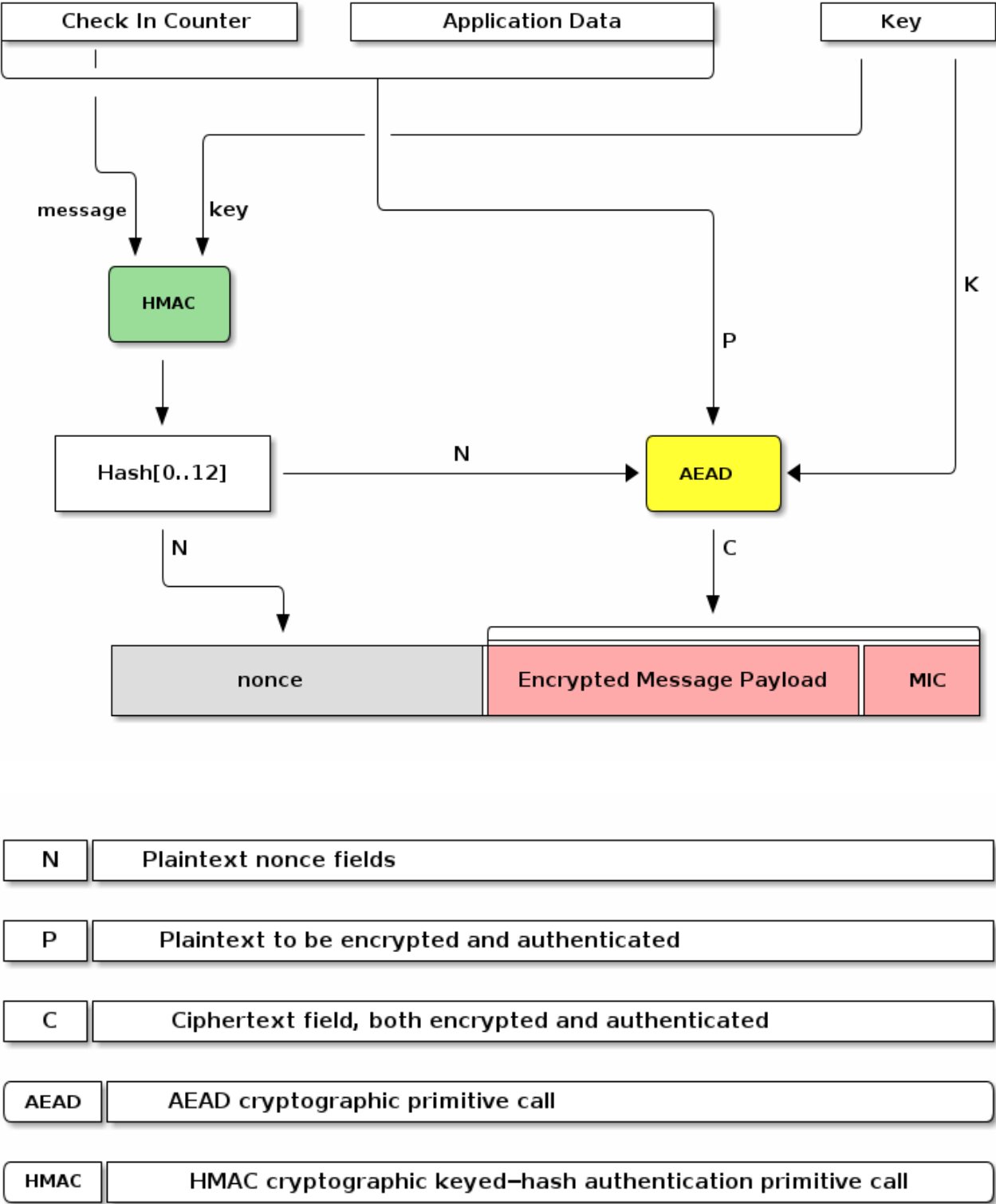
Figure 29. Check-In Protocol Encryption Legend
