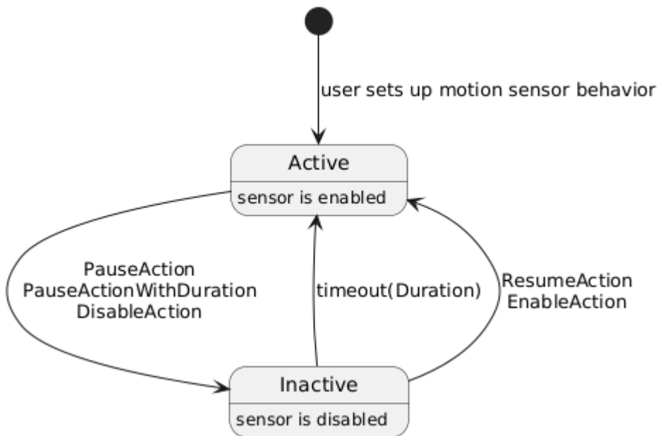
Figure 67. State diagram for example 'pause sensor automation'
