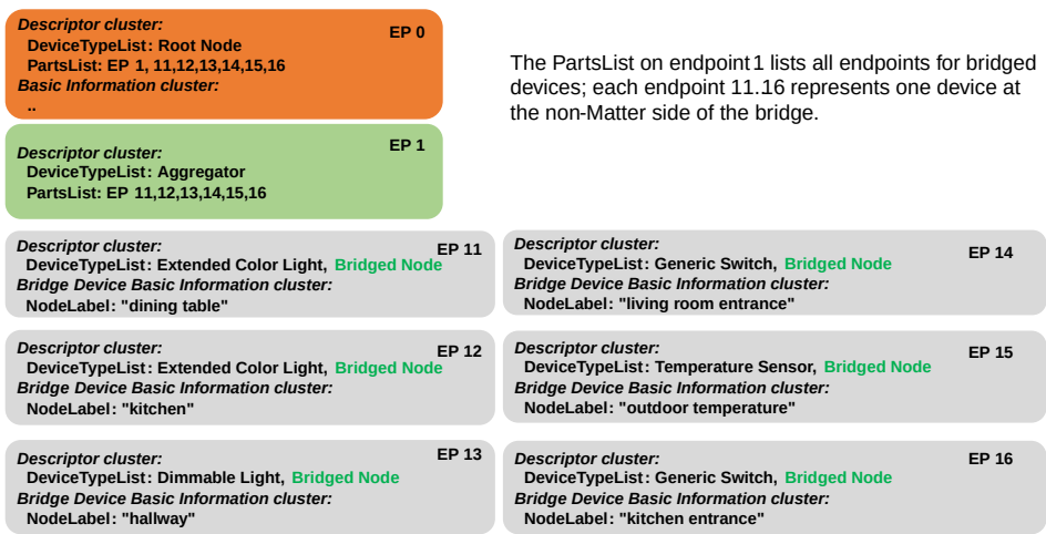
Figure 58. example of endpoints representing Bridged Devices
