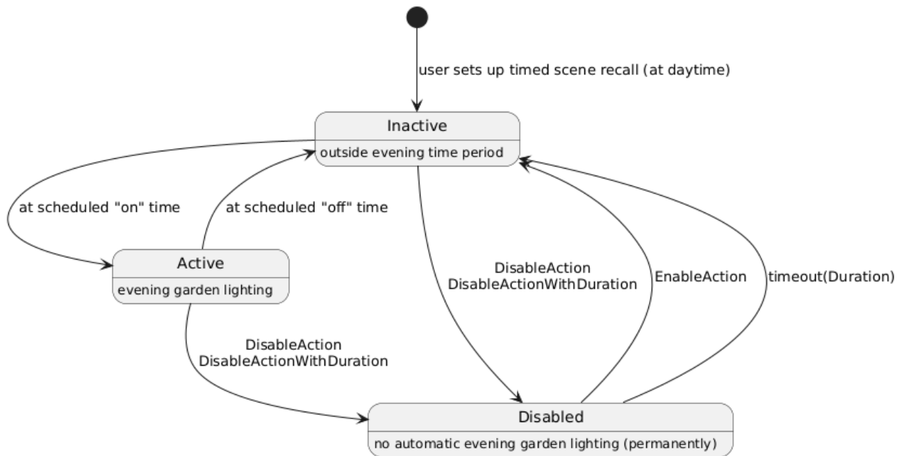
Figure 69. State diagram for example 'scheduled scene recall'
