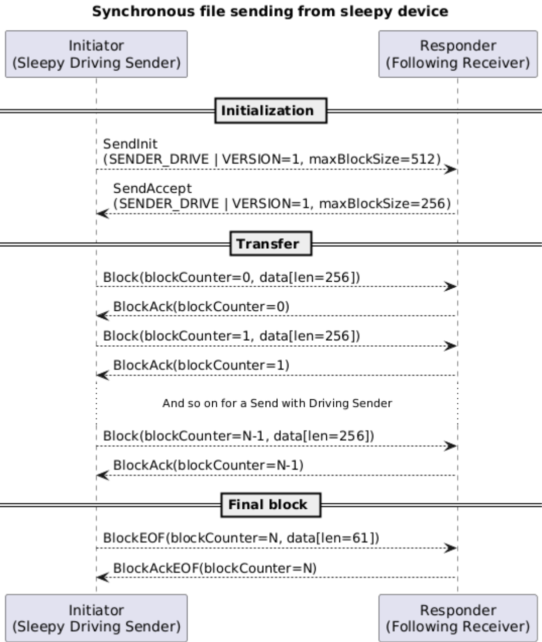
Figure 92. Synchronous file sending from sleepy device acting as driving Sender
