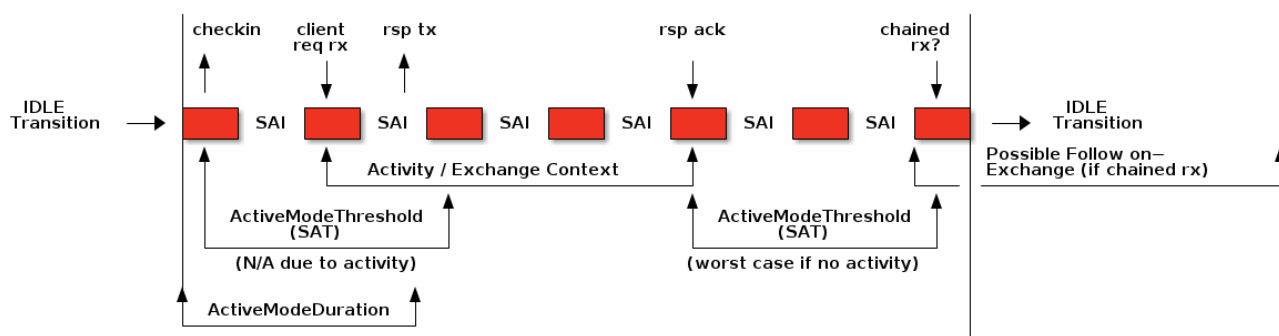
Figure 73. ICD Active Mode Behavior Diagram
