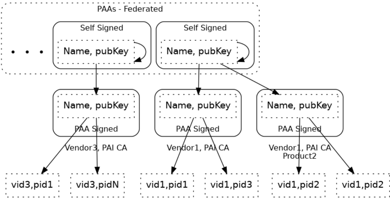
Figure 46. Device Attestation PKI hierarchy
