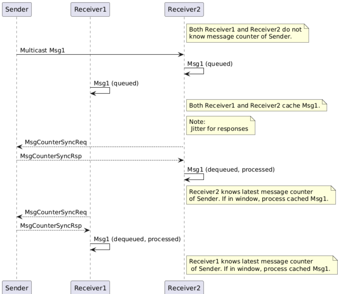
Figure 21. Multicast Receiver Initiated Message Counter Synchronization
