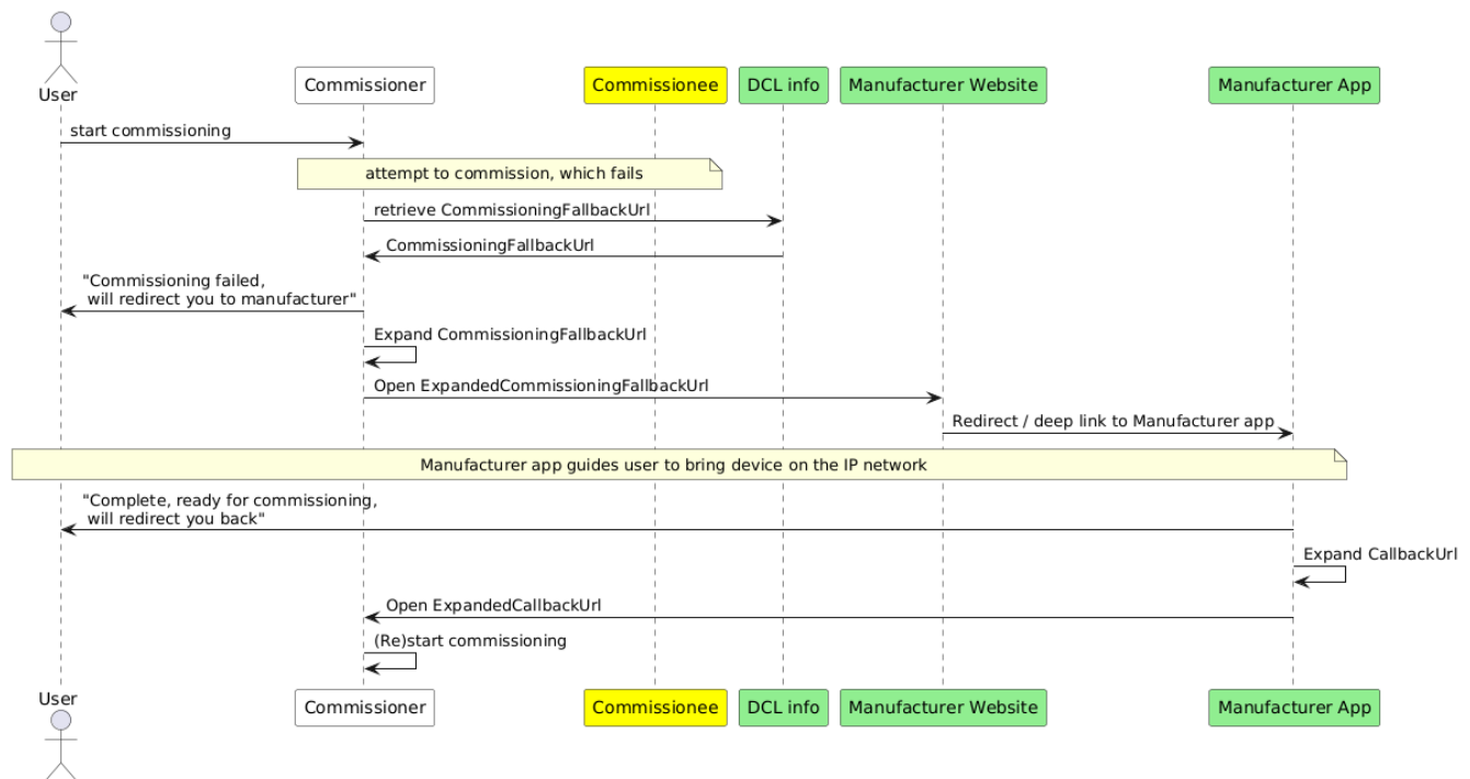
Figure 45. Commissioning Fallback Mechanism sequence diagram
