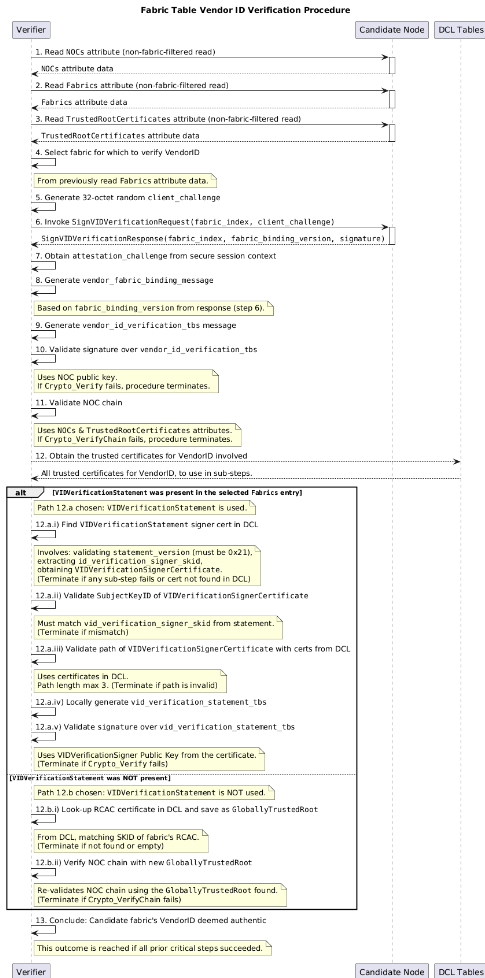
Figure 51. Sequence diagram of Fabric Table Vendor ID Verification Procedure
